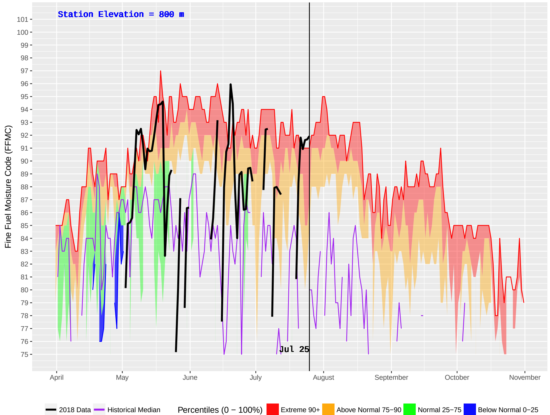
DEASE LAKE FS (108) : Historical (1978–2016) and Current (2018) Noon Fine Fuel Moisture Code (FFMC)
