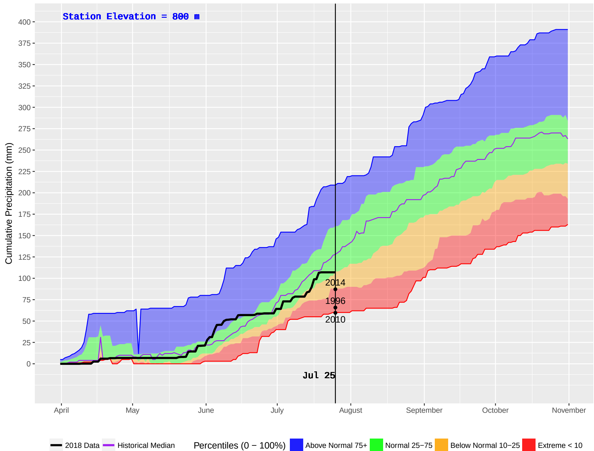
DEASE LAKE FS (108) : Historical (1978–2016) and Current (2018) Noon Cumulative Precipitation
